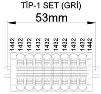
HYBRIT TYPE TERMINAL BLOCK PUSH-IN TO SCREW CONNECTION
