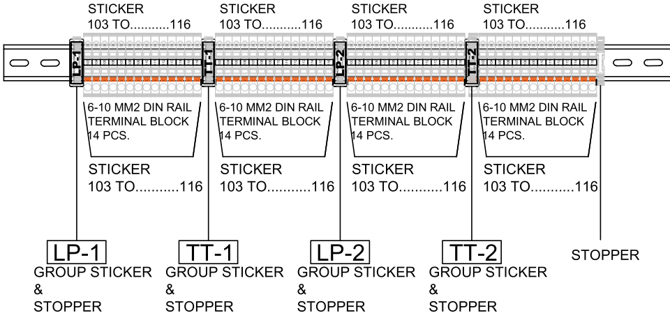
HYBRIT TYPE TERMINAL BLOCK PUSH-IN TO SCREW CONNECTION
